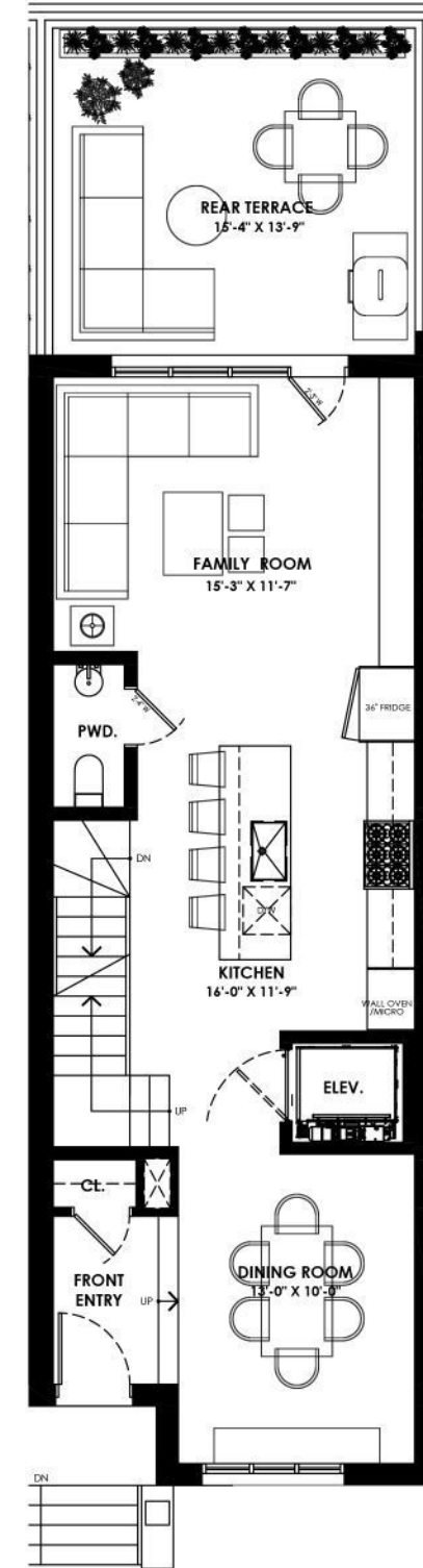
UNIT 3 MAIN LEVEL
