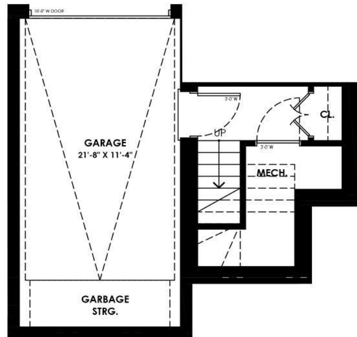
UNIT 6 BASEMENT
