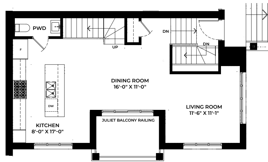
UNIT 7 MAIN LEVEL
