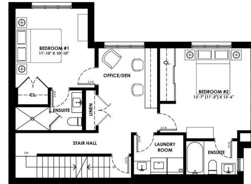
UNIT 6 SECOND LEVEL
