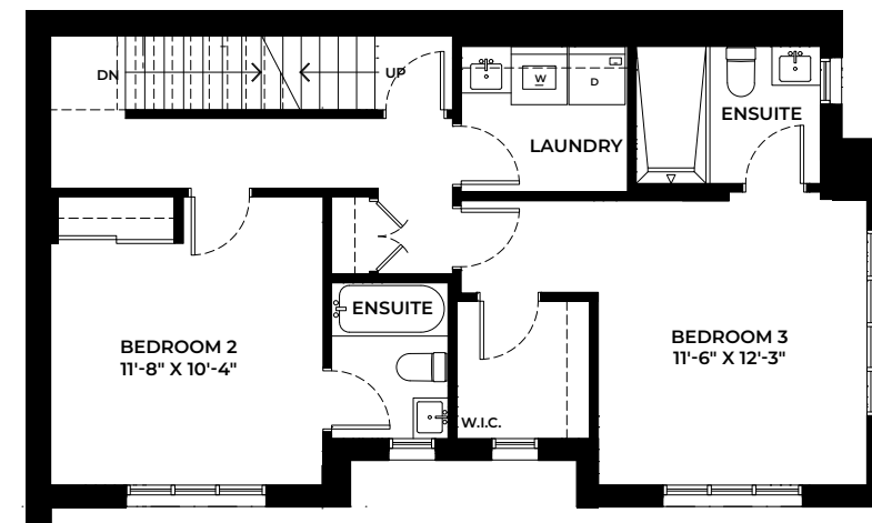
UNIT 7 SECOND LEVEL
